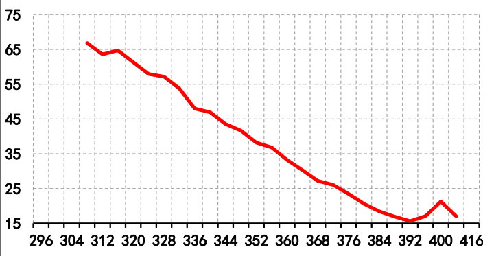
沪金看跌期权隐含波动率 202006
